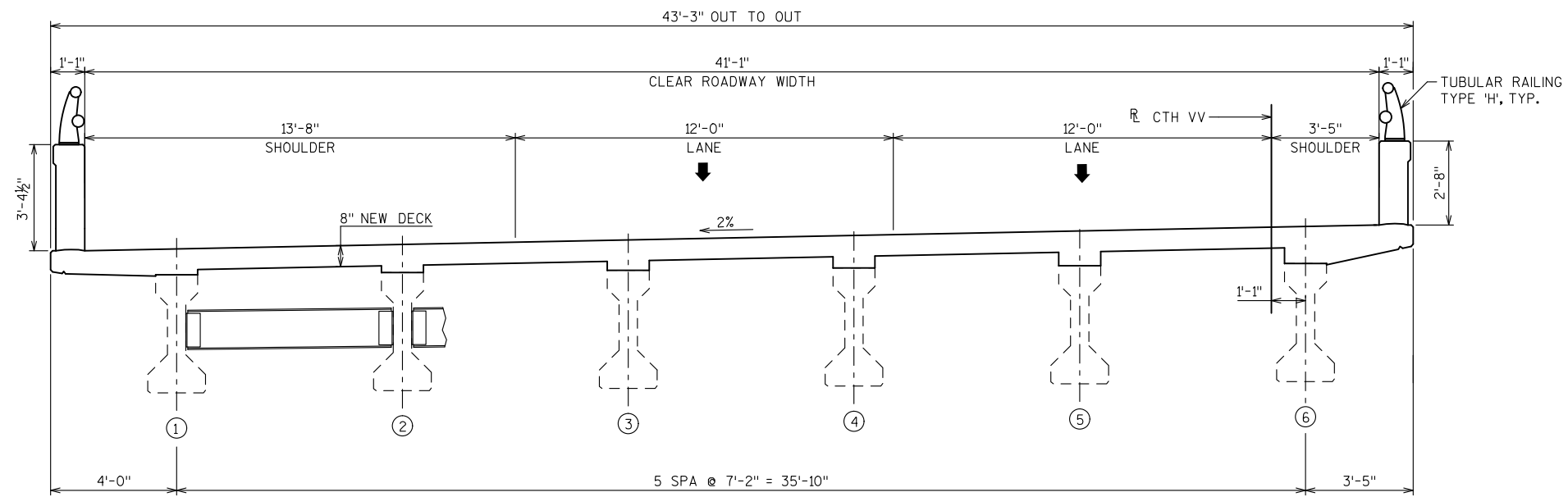
CTH VV WB EXISTING TYPICAL SECTION AT BRIDGE (LOOKING EAST)
