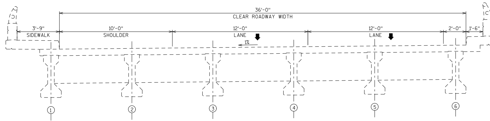
CTH VV WB EXISTING TYPICAL SECTION AT BRIDGE (LOOKING EAST)
