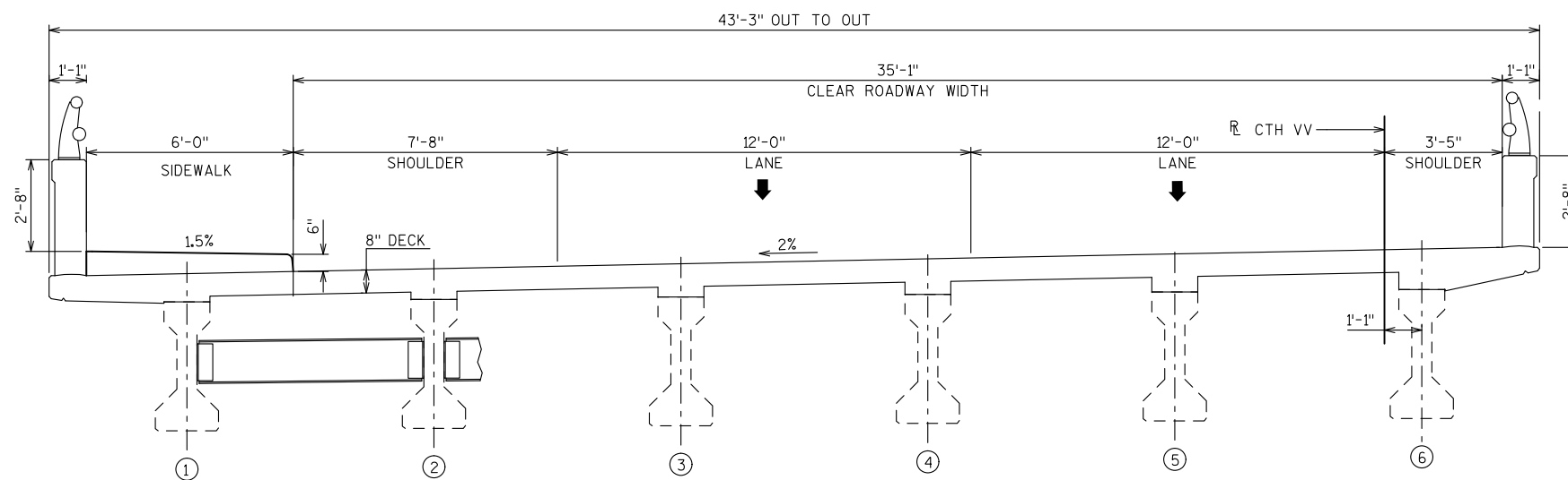
CTH VV WB PROPOSED TYPICAL SECTION AT BRIDGE (LOOKING EAST)
